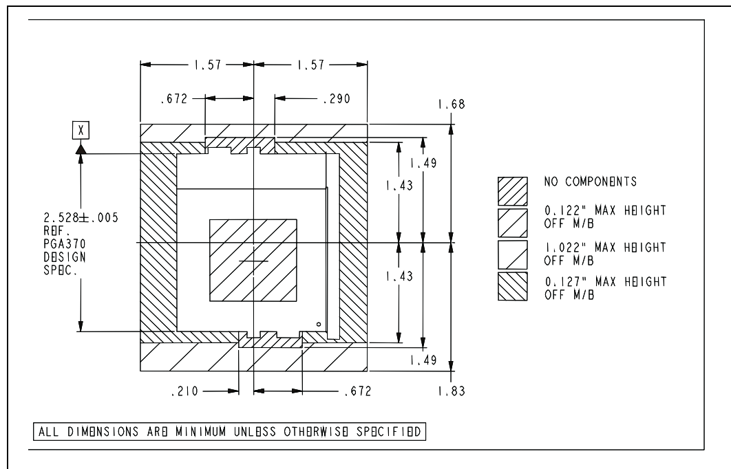
Figure 30. Component Keep-Out
