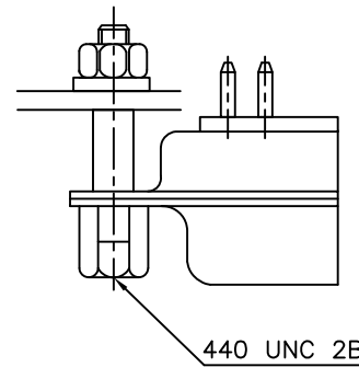
EXTENDED FEMALE SCREW LOCK WITH SPACER
