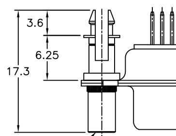
UNC 4-40 OPTION:-V with G
