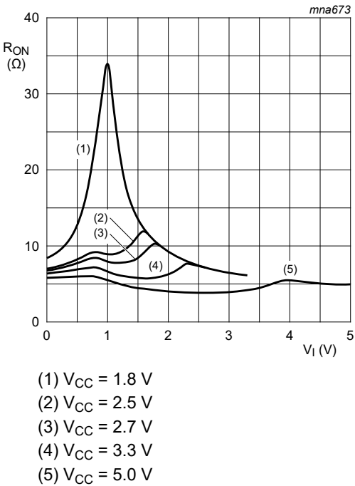
Fig. 9. Typical ON resistance as a function of input voltage; T_{amb} = 25 \text{ }^{\circ}\text{C}
