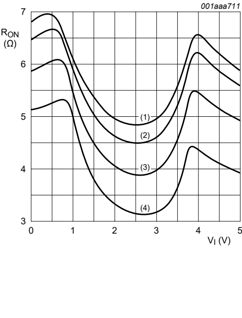
Fig. 14. ON resistance as a function of input voltage; V_{CC} = 5.0 V
