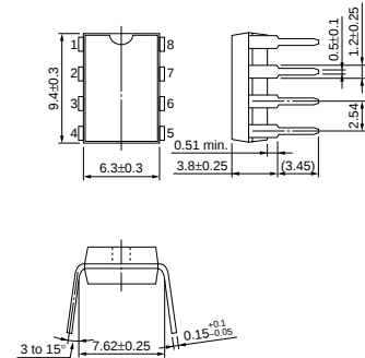
DIP008-P-0300B
