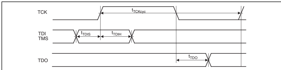
Figure 31.65 H-UDI Data Transfer Timing
