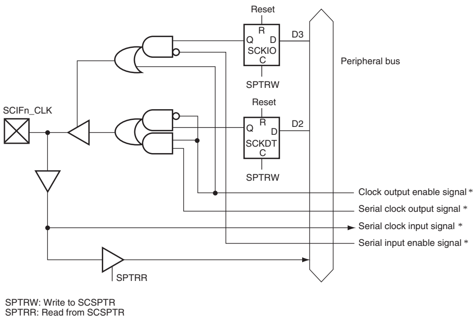
Figure 21.4 SCIF n _SCK Pin (n = 0, 1)
