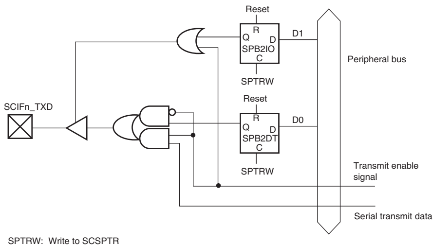
Figure 21.5 SCIFn_TXD Pin (n = 0, 1)
