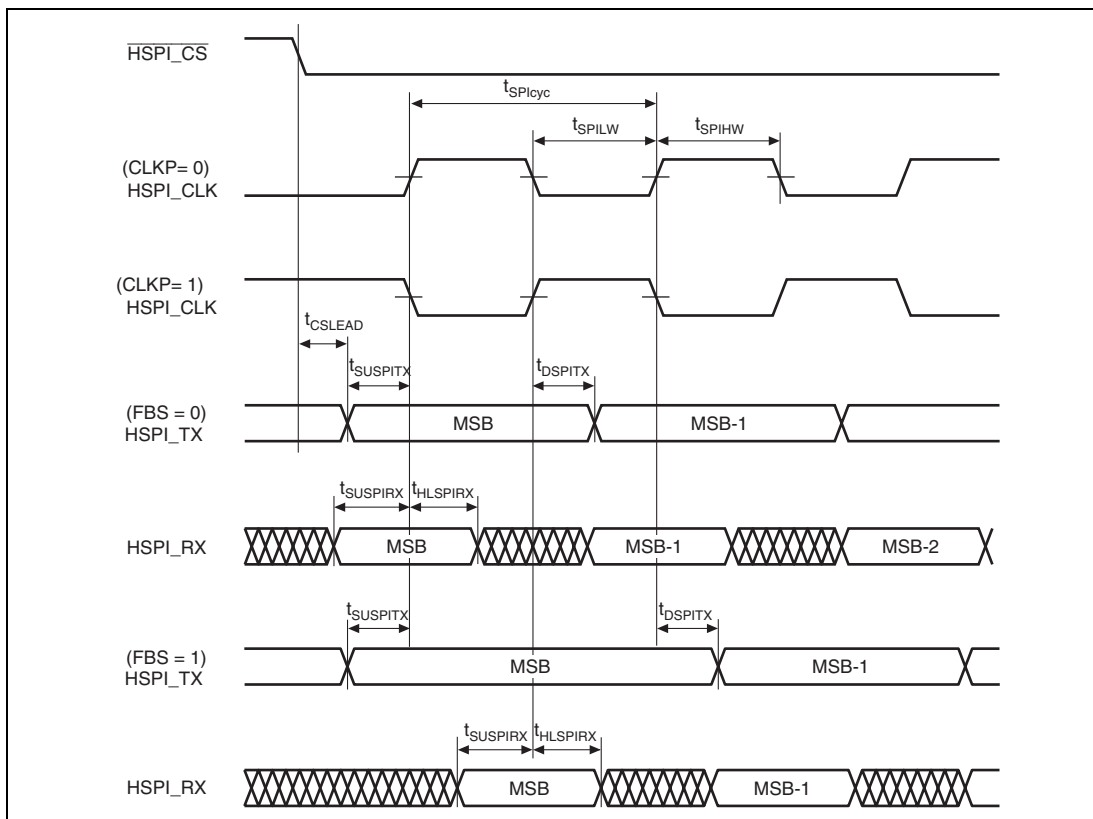
Figure 31.45 HSPI Data Output/Input Timing
