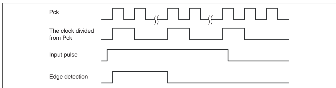
Figure 19.2 Edge Detection (example of rising edge)
