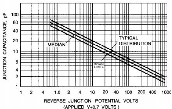
Fig. 2 - JUNCTION CAPACITANCE
