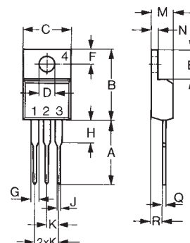
Outlines TO-220
