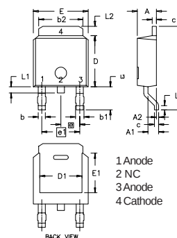
Outlines TO-252 AA
