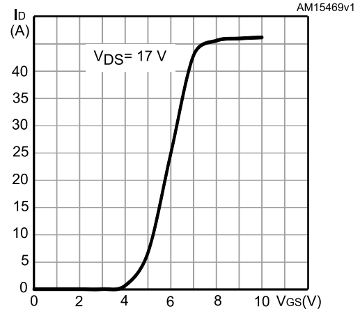
Figure 5: Transfer characteristics
