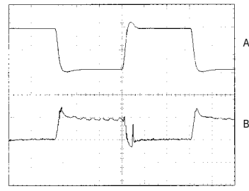
MAX649 LOAD-TRANSIENT RESPONSE
