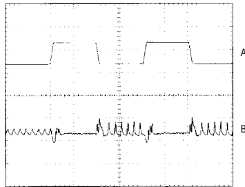
MAX649 LINE-TRANSIENT RESPONSE
