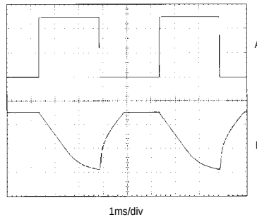
MAX649 SHUTDOWN RESPONSE TIME
