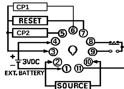
H7CN-□□□M Counter
