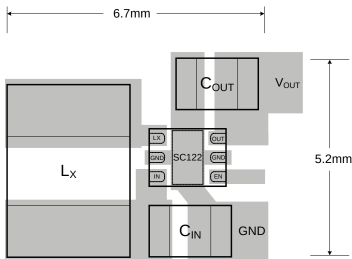
Figure 2 — Recommended Layout
