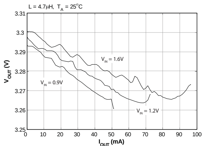
Load Regulation
