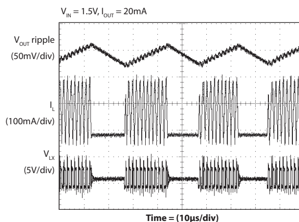
Figure 1 — PSAVE Regulation Waveforms
