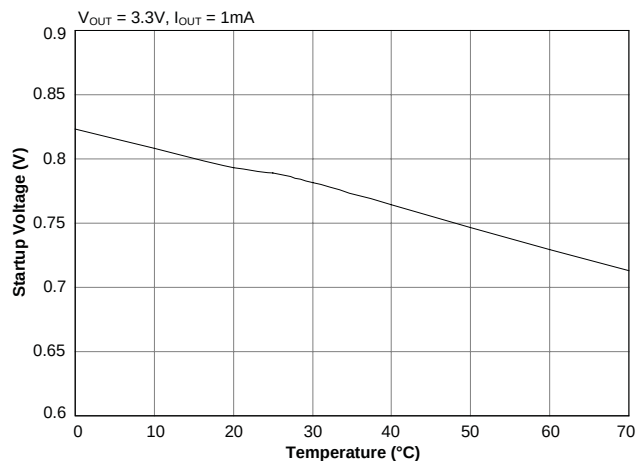
Minimum Start-up Voltage vs. Temperature
