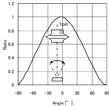
Fig.4 Directional Characteristics 1
