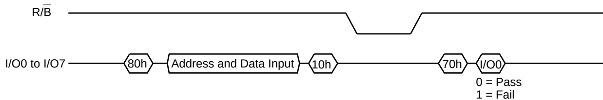
Figure 5 Page Program
