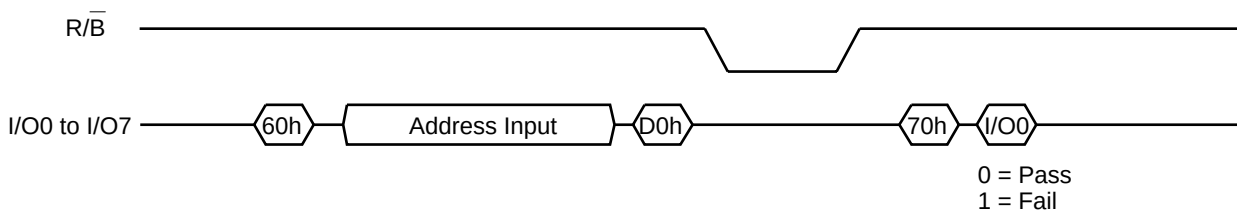
Figure 6 Block Erase
