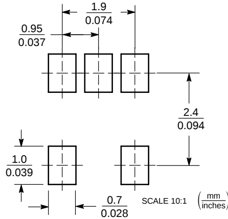
Figure 15. THIN SOT23-5/TSOP-5/SC59-5
