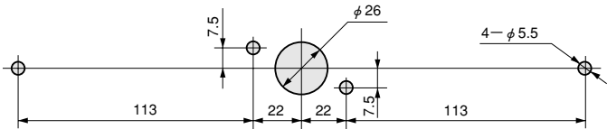
Layout of Holes for Installation
