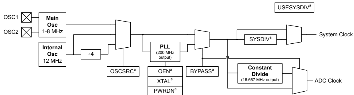
Figure 6-4. Main Clock Tree
