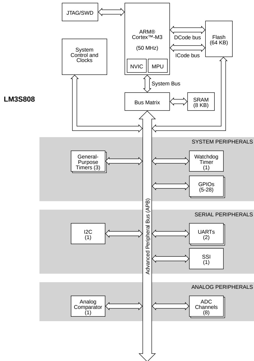
Figure 1-1. Stellaris® LM3S808 Microcontroller High-Level Block Diagram
