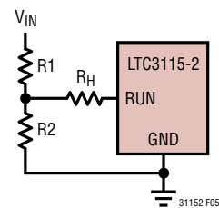
Figure 5. Increasing Input UVLO hysteresis
