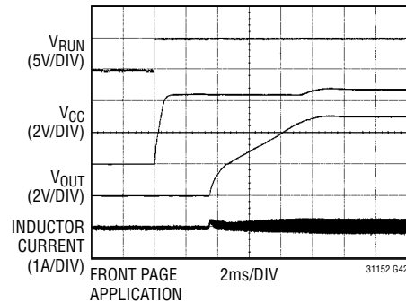
Soft-Start Waveforms
