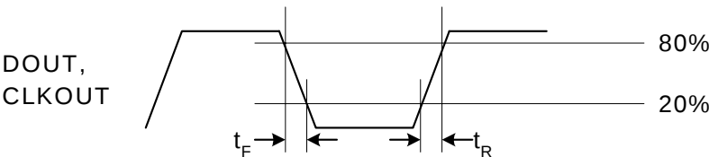
Figure 3. DOUT and CLKOUT Rise/Fall Times
