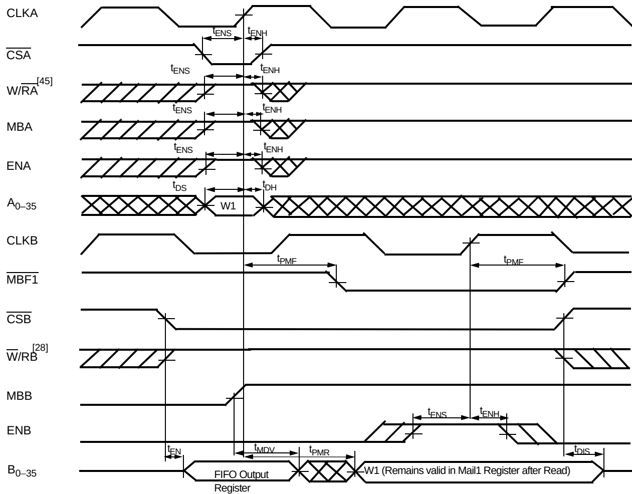
Timing for Mail1 Register and MBF1 Flag (CY Standard and FWFT Modes) [44]
