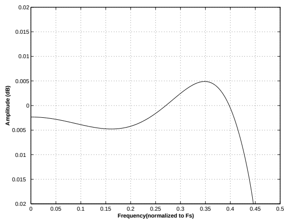
Figure 57. Double-Speed (fast) Passband Ripple
