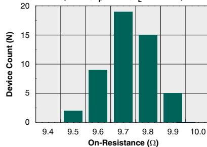
Typical On-Resistance Distribution (N=50, I_F=5\text{mA} , I_L=150\text{mA} )
