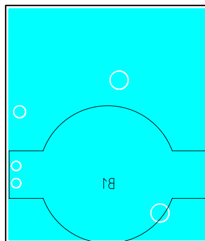
Figure 4-2 Top Side of TDK 5110-Testboard with 50 \Omega -Output
