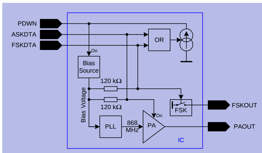
Figure 3-5 Power mode control circuitry
