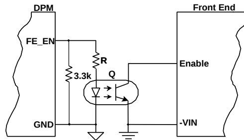
Figure 17. Interface between DPM and DC-DC Front End
