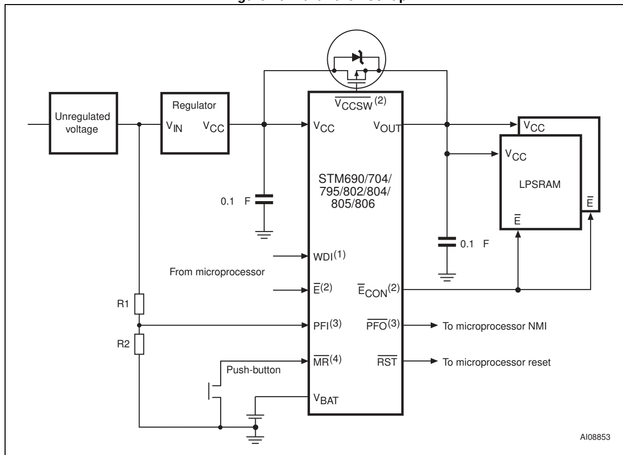
Figure 10. Hardware hookup
