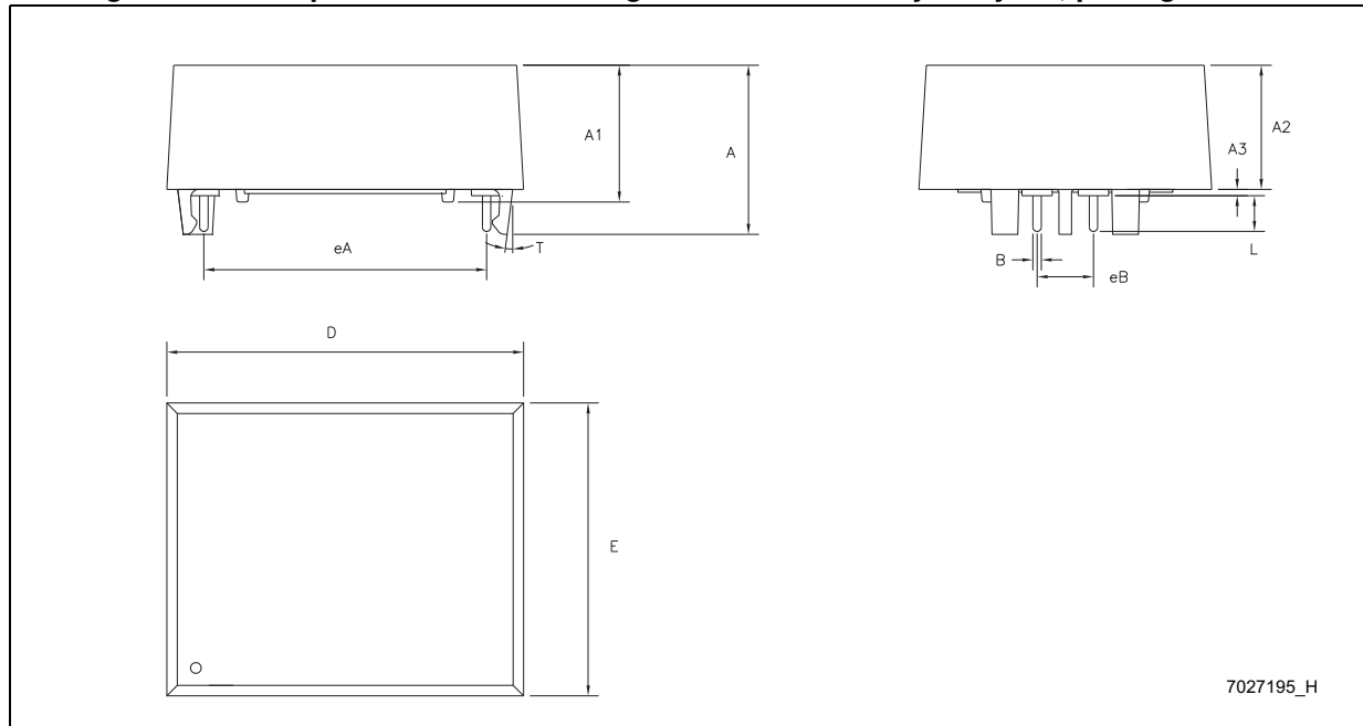
Figure 6. SH – 4-pin SNAPHAT® housing for 120 mAh battery &amp; crystal, package outline
