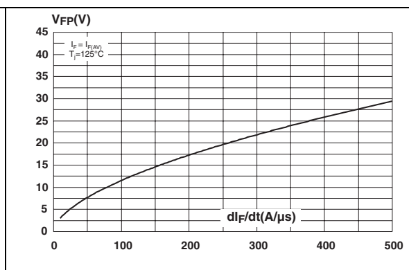
Figure 10. Transient peak forward voltage versus dl_F/dt (typical values)
