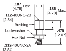
Part Number 6-1532137-4 Jackpost Assembly (S) S96-0002-0060 M83513/5-17
