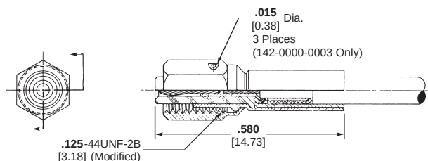
Straight Plug 1
