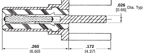
Straight Printed Circuit Receptacle Mounting Hole Pattern Shown Below Part Number 141-1004-0001
