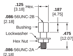
Part Number 5-1532137-9 Jackpost Assembly (P) S96-0002-0009 M83513/5-07
