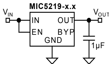
Figure 5. Low-Noise Fixed Voltage Regulator
