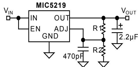
Figure 8. Ultra-Low-Noise Adjustable Application
