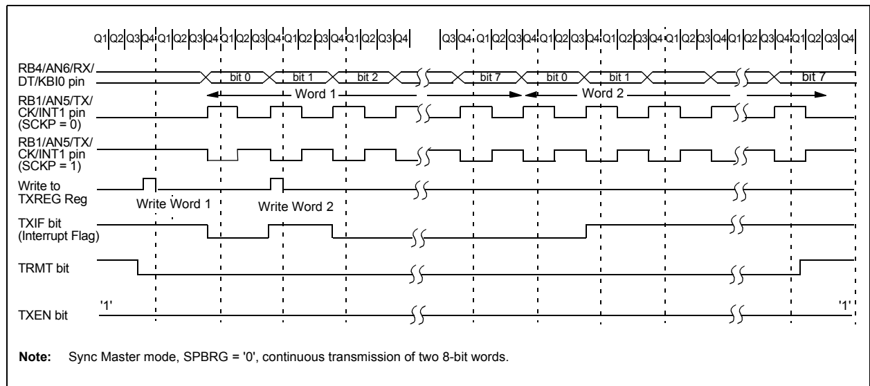
FIGURE 16-10: SYNCHRONOUS TRANSMISSION
