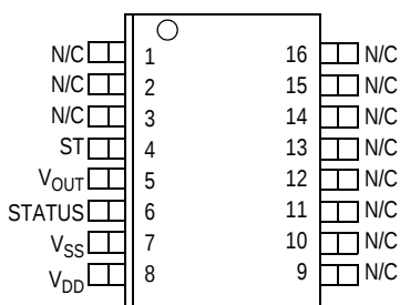
Figure 2. Pin Connections
