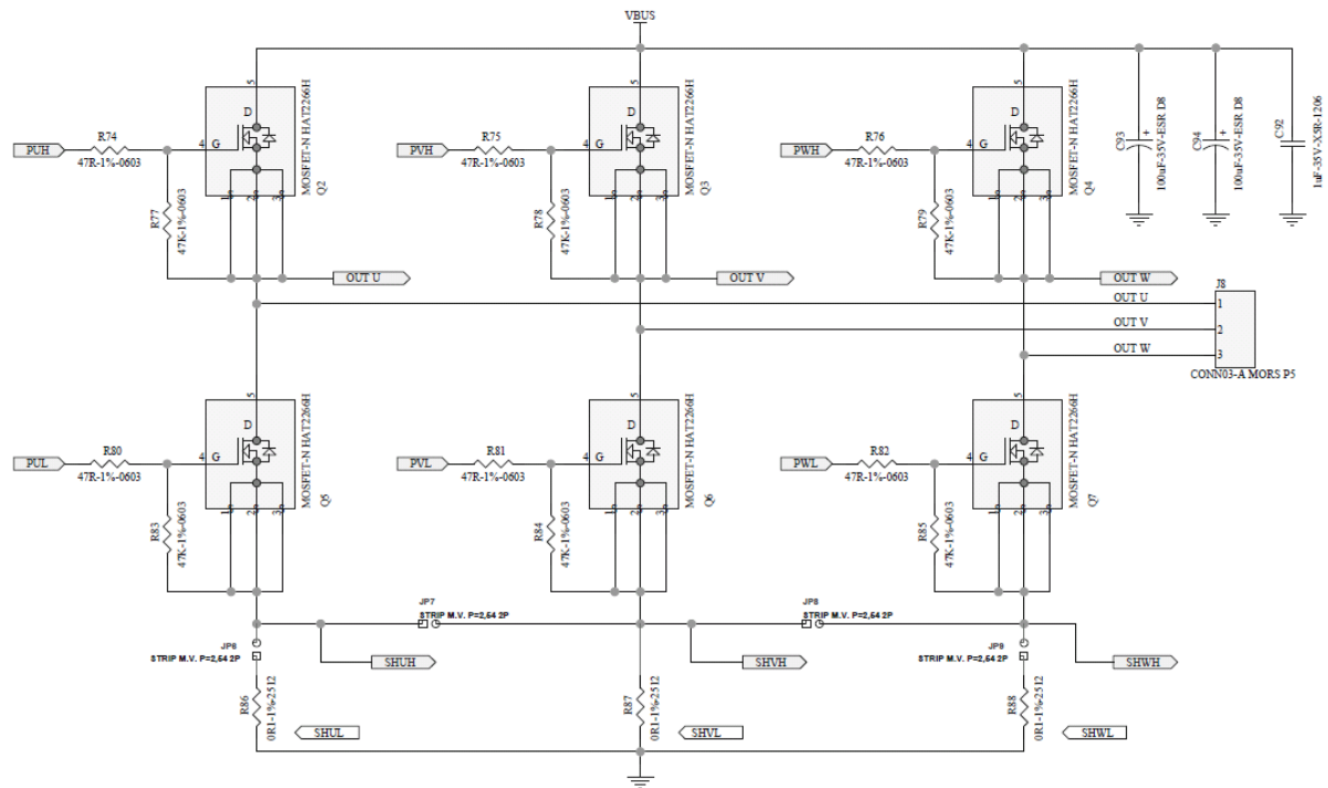
Figure 4 H-Bridge
