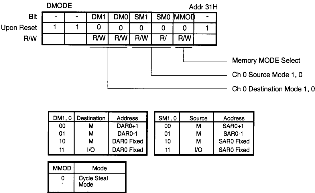
Figure 55. DMA Mode Registers
