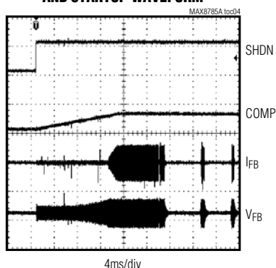
MINIMUM BRIGHTNESS OPERATION AND STARTUP WAVEFORM
