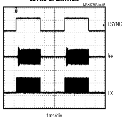
LSYNC OPERATION
