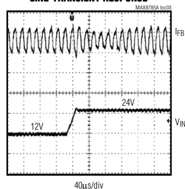
LINE-TRANSIENT RESPONSE
