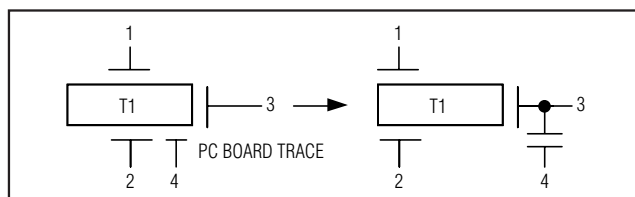
Figure 7. Arc Protection
