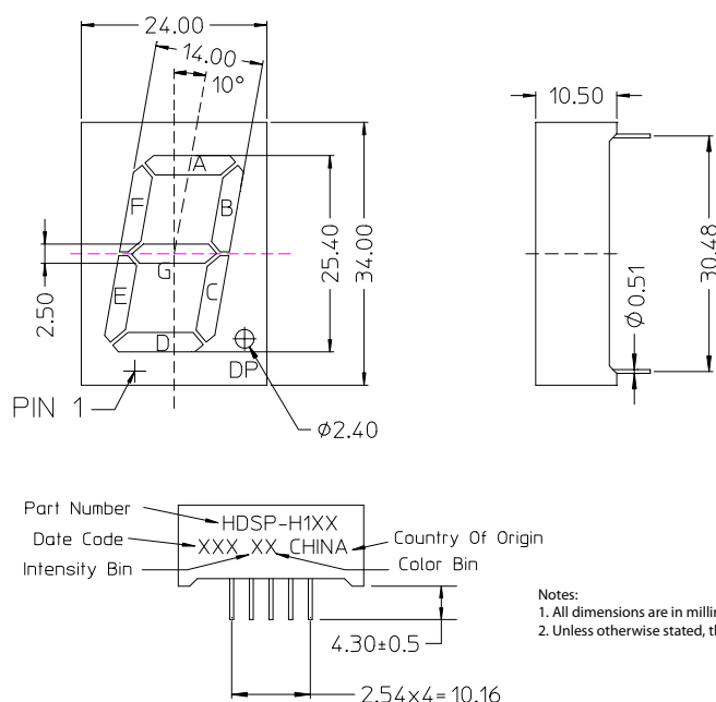
Figure 1 Package Dimension
