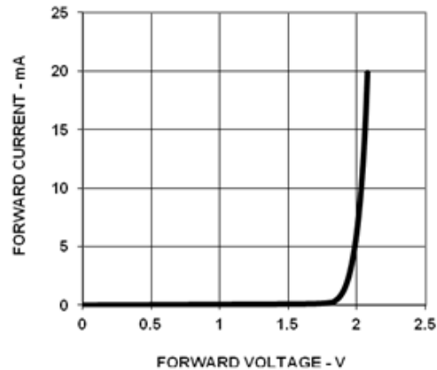
Figure 9 Forward Voltage Vs Current (DP)
