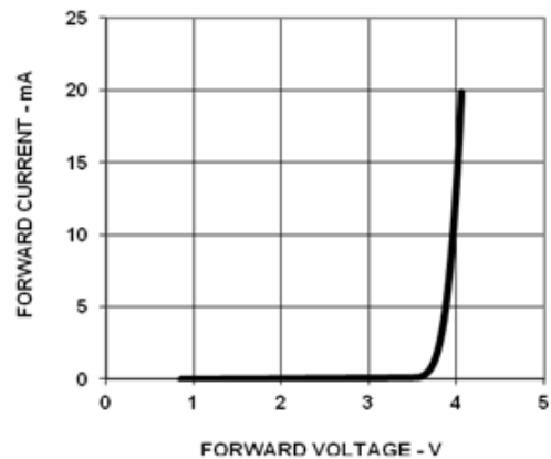
Figure 8 Forward Voltage Vs Current (Segment)
