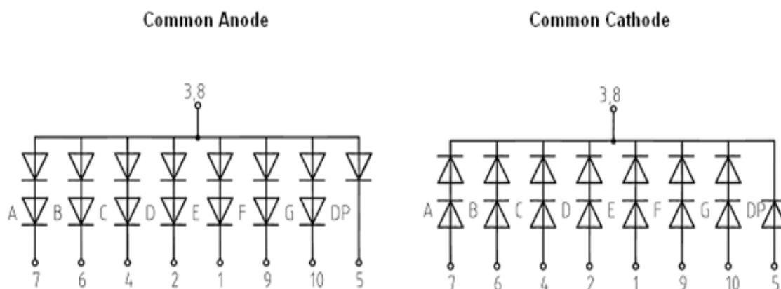
Figure 2 Circuit Diagram
