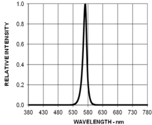
Figure 10 Relative Luminous Intensity Vs Wavelength
