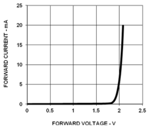
Figure 13 Forward Voltage Vs Current (DP)
