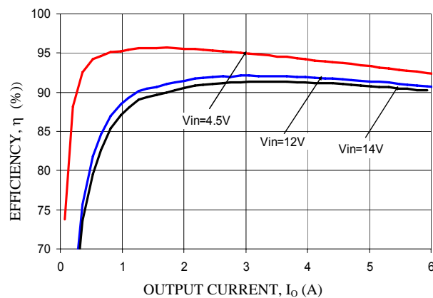
V_o = 3.3V
