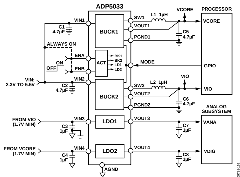
Figure 47. Processor System Power Management with PSM/PWM Control
