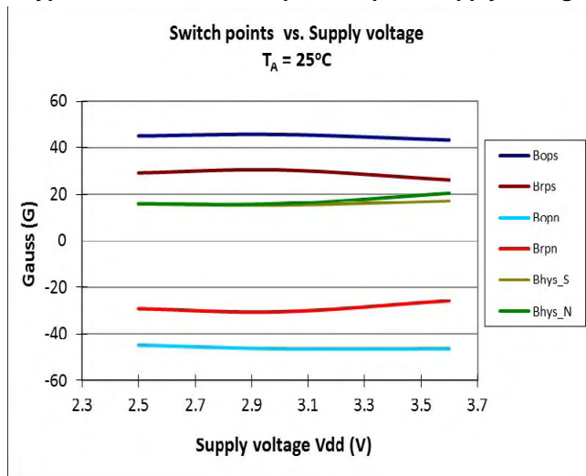
Typical Switch Points Bop and Brp vs. Supply Voltage
