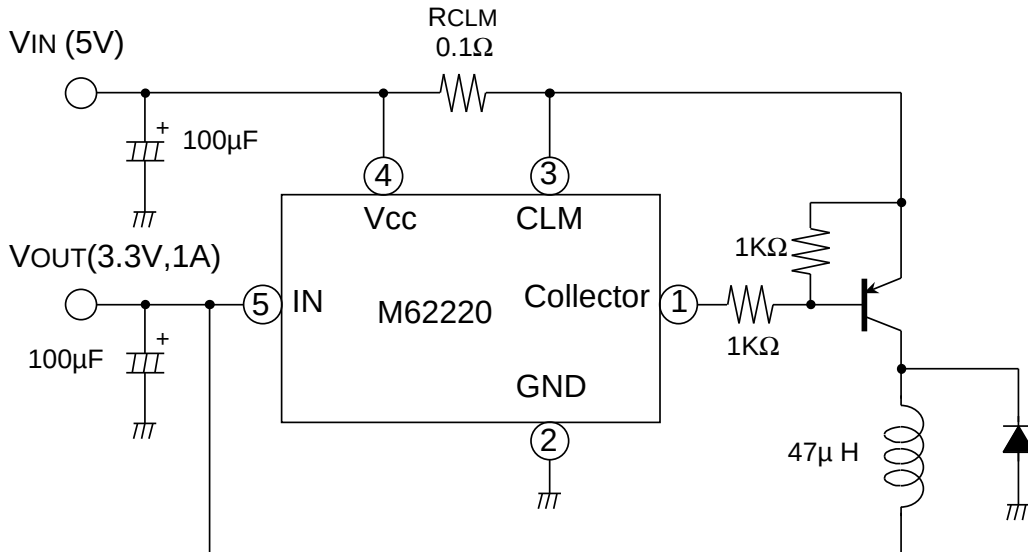
Fig.1 Example of the M62220L/FP application circuit
