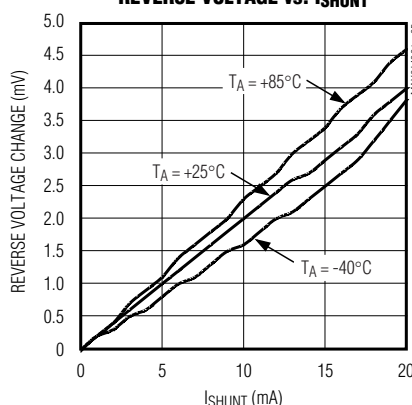
MAX6138_12 REVERSE VOLTAGE vs. I_{SHUNT}
