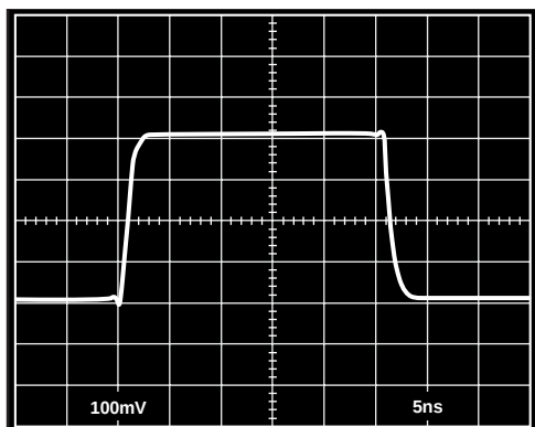
Figure 13. AD9632 Small Signal Transient Response; V_{OUT} = 400\text{ mV p-p} , G = +2 , R_F = R_{IN} = 274\ \Omega
