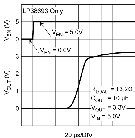
Figure 28. V_{\text{OUT}} vs V_{\text{EN}} , ON (LP38693 Only)
