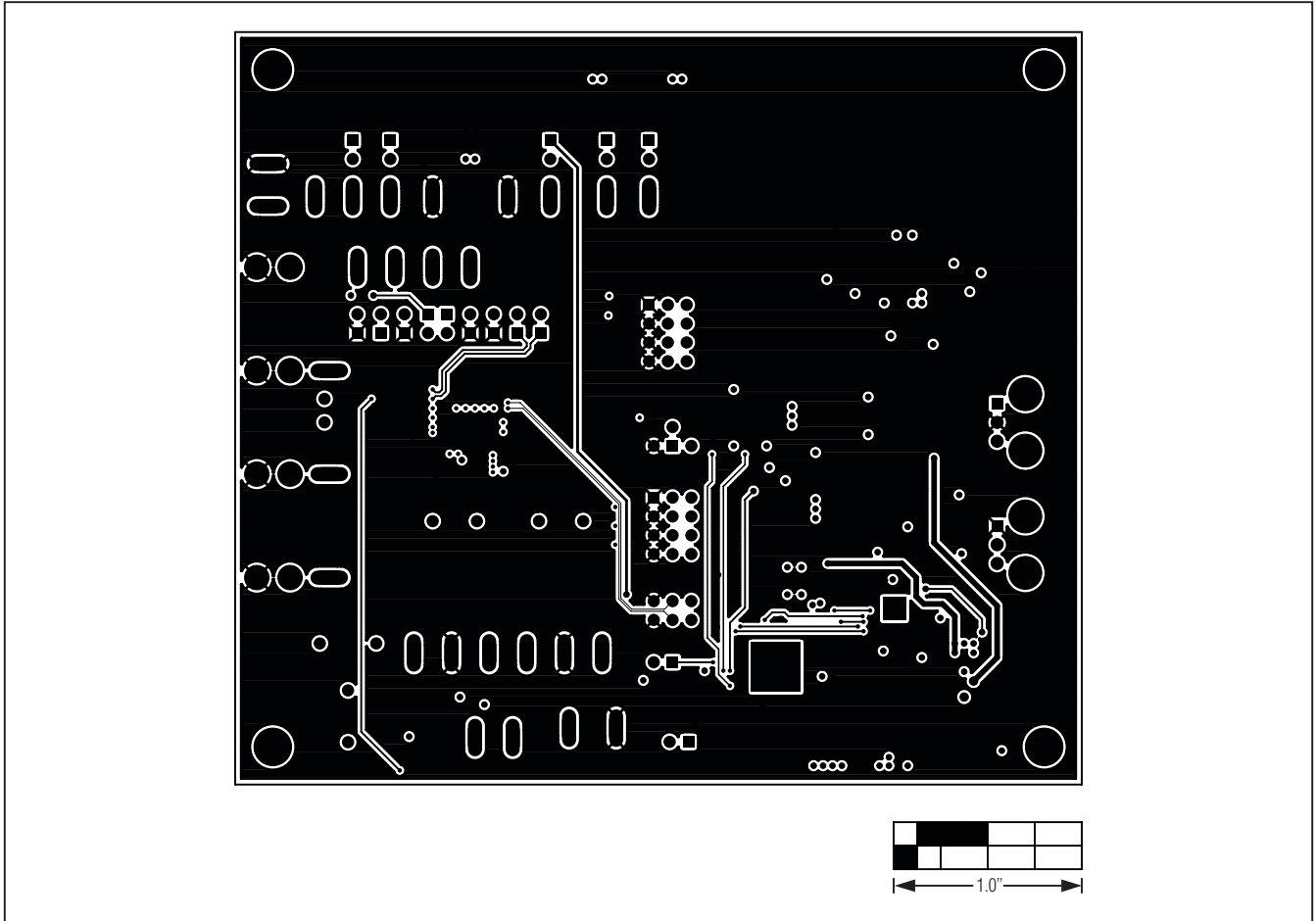
Figure 11. MAX98088 EV Kit PCB Layout—Solder Side
