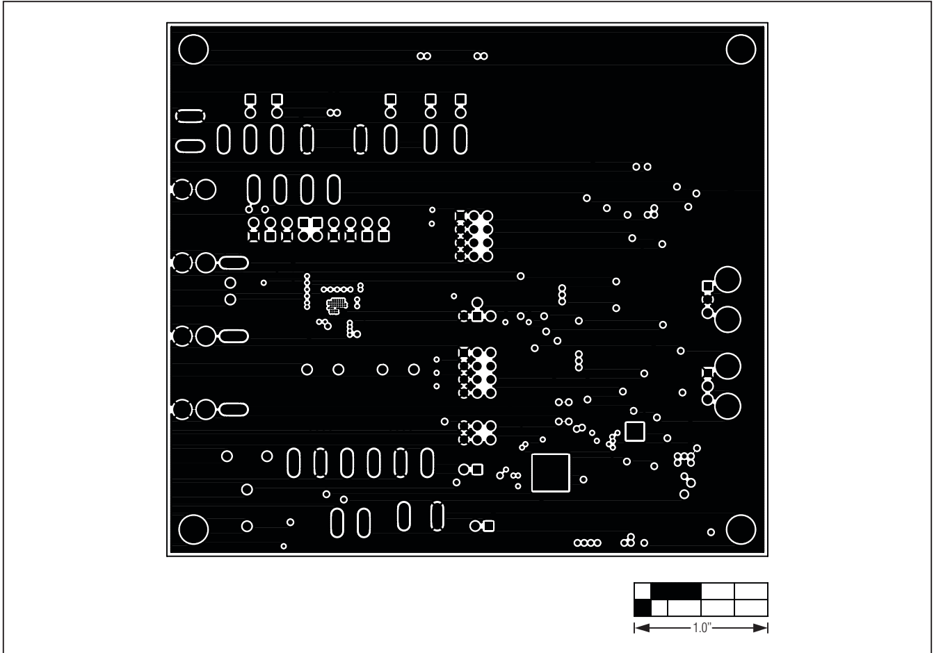
Figure 7. MAX98088 EV Kit PCB Layout—Ground Layer 2
