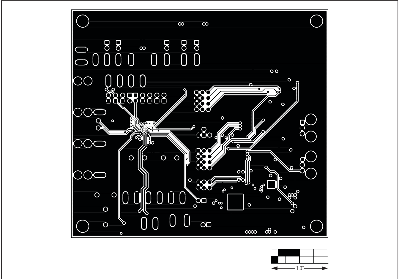
Figure 8. MAX98088 EV Kit PCB Layout—Ground Layer 3
