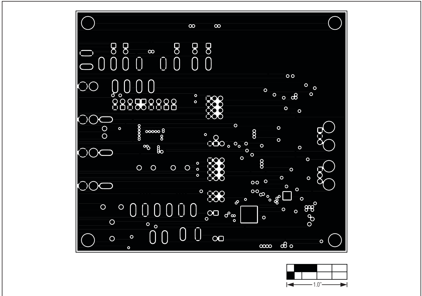
Figure 10. MAX98088 EV Kit PCB Layout—Ground Layer 5
