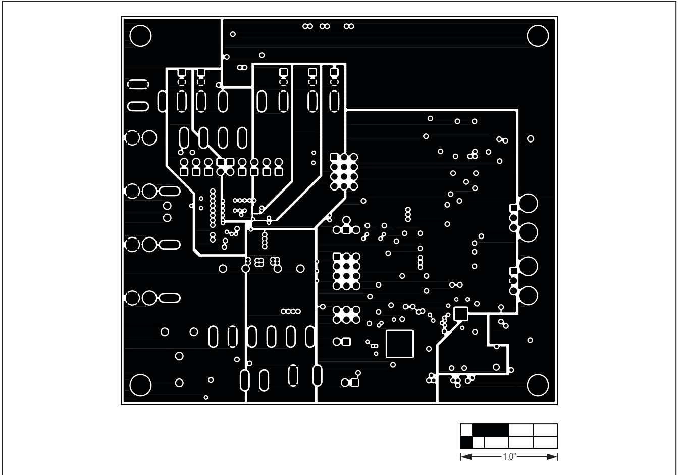
Figure 9. MAX98088 EV Kit PCB Layout—Power Layer 4
