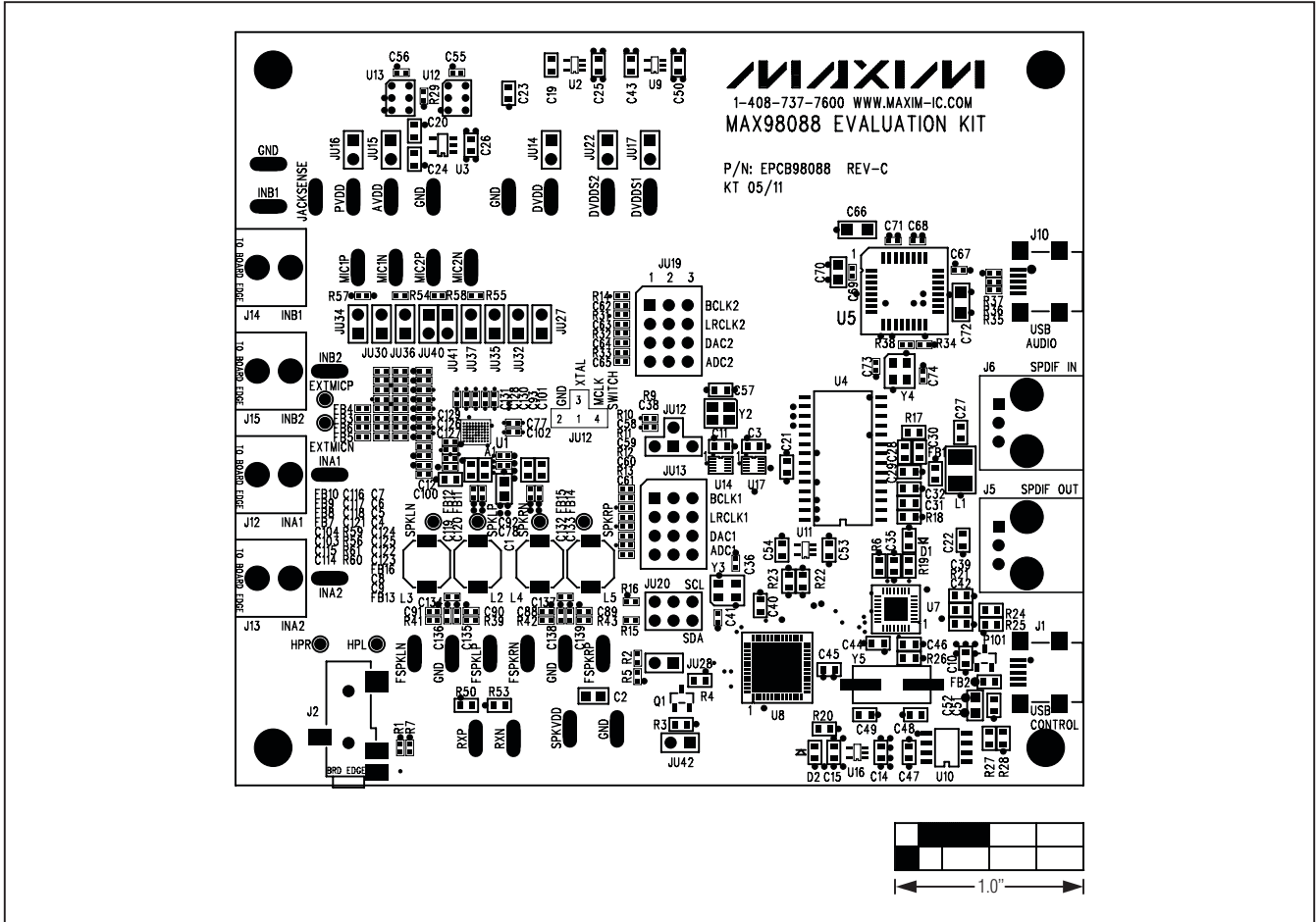
Figure 5. MAX98088 EV Kit Component Placement Guide—Component Side
