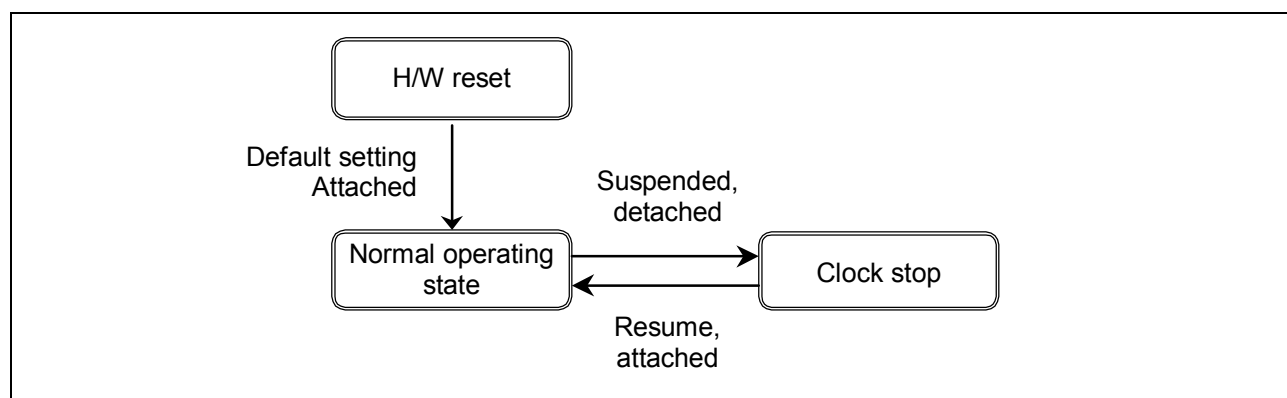
Figure 3.4 Controller state transitions (using clock stop state)
