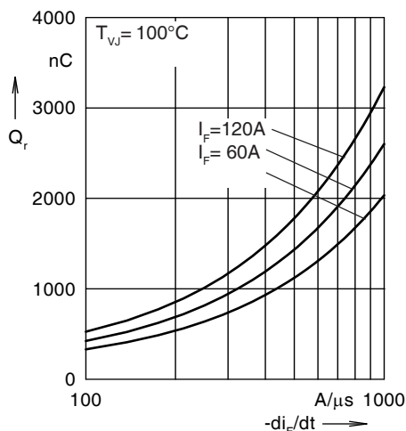
Fig. 19. Reverse recovery charge Q_r
