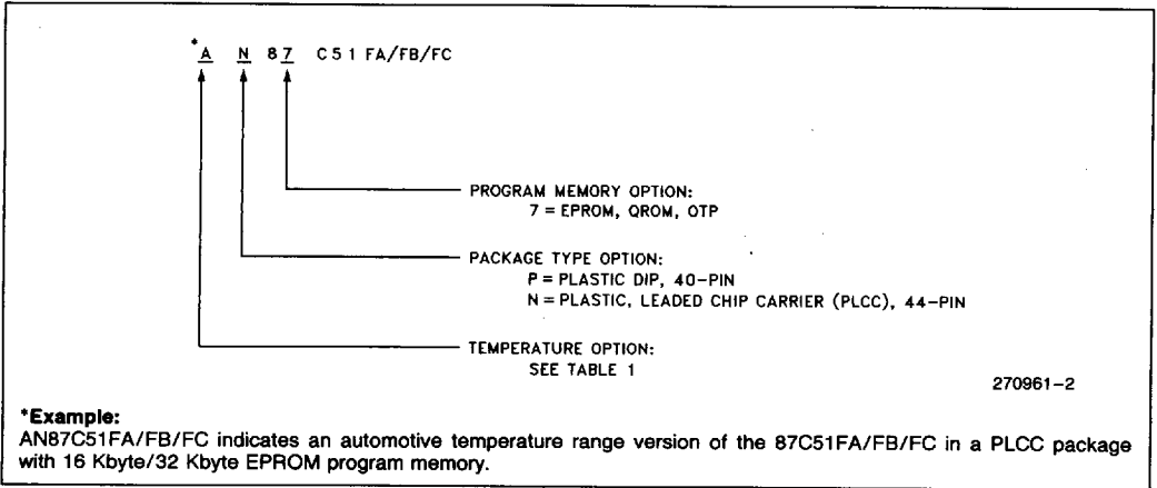
Figure 2. Package Options
