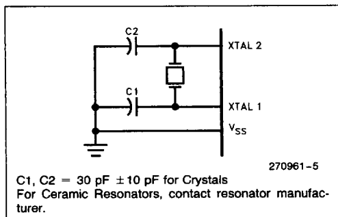
Figure 4. Oscillator Connections
