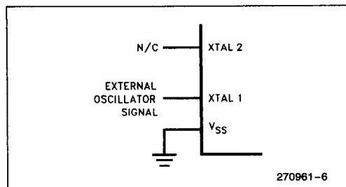
Figure 5. External Clock Drive Configuration
