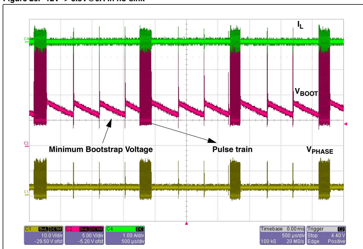
Figure 26. 12V \rightarrow 3.3V@0A in no-sink
