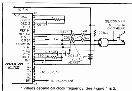
Figure 11. 7126 used as a Digital Centigrade Thermometer. A silicon diode-connected transistor has a temperature coefficient of about -2\text{mV}/^\circ\text{C} . Calibration is achieved by placing the sensing transistor in ice water and adjusting the zeroing potentiometer for a 000.0 reading. The sensor should then be placed in boiling water and the scale-factor potentiometer adjusted for a 100.0 reading.
