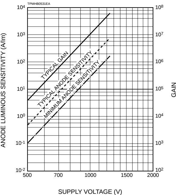
Figure 2: Anode Sensitivity and Gain Characteristics
