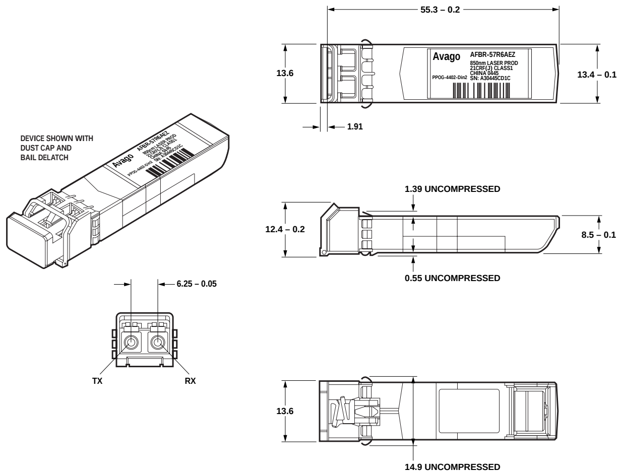
Figure 5. Module drawing
