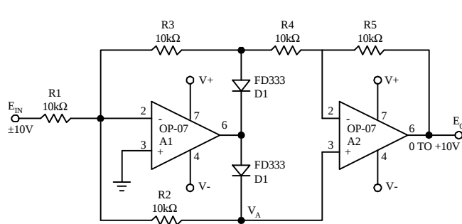
Precision Absolute Value Circuit
