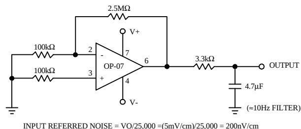
TYPICAL LOW-FREQUENCY NOISE TEST CIRCUIT
